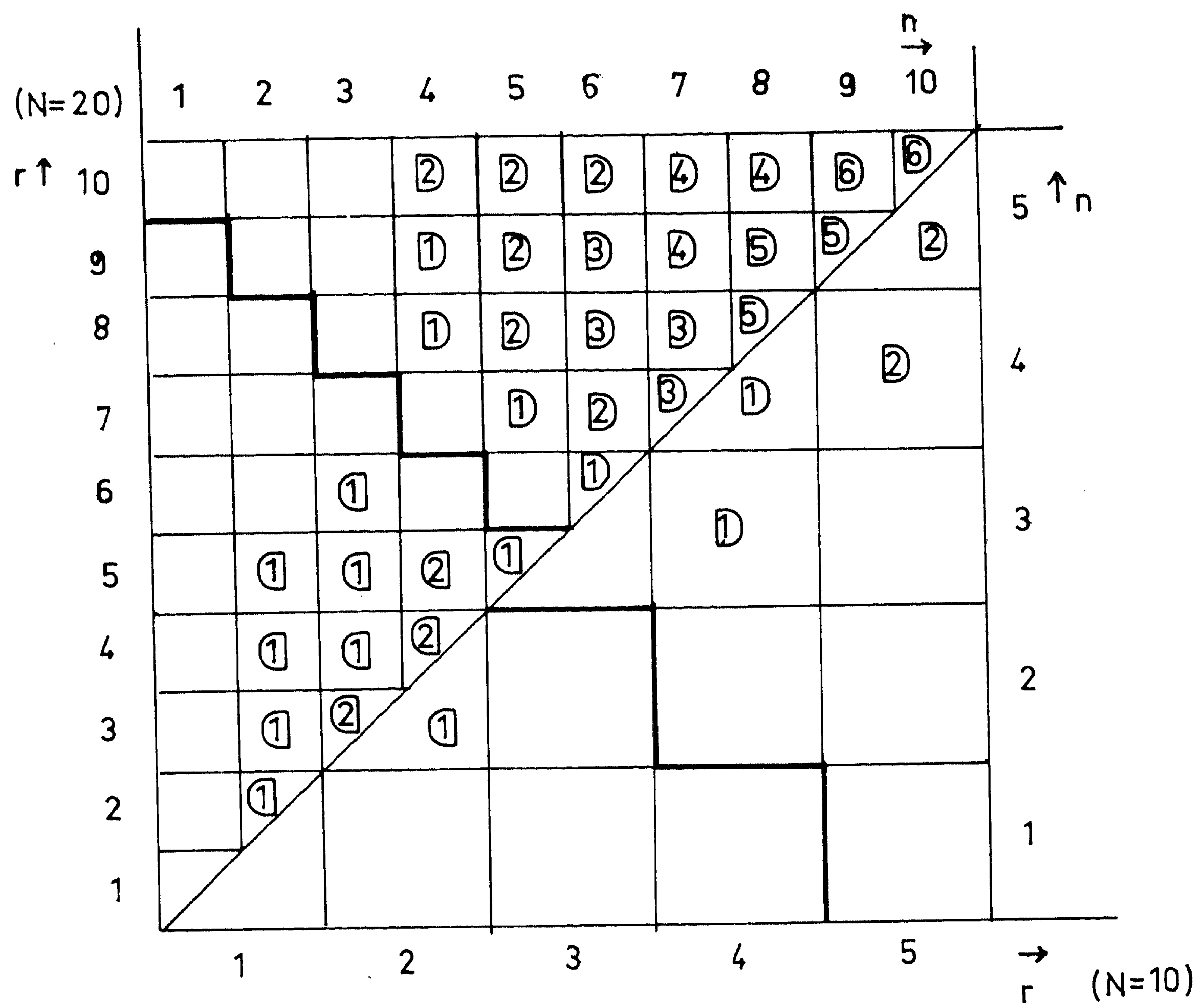
Fig. 1. \square : normal approx. better \square : \chi^2 approx. better N = 10, 20
